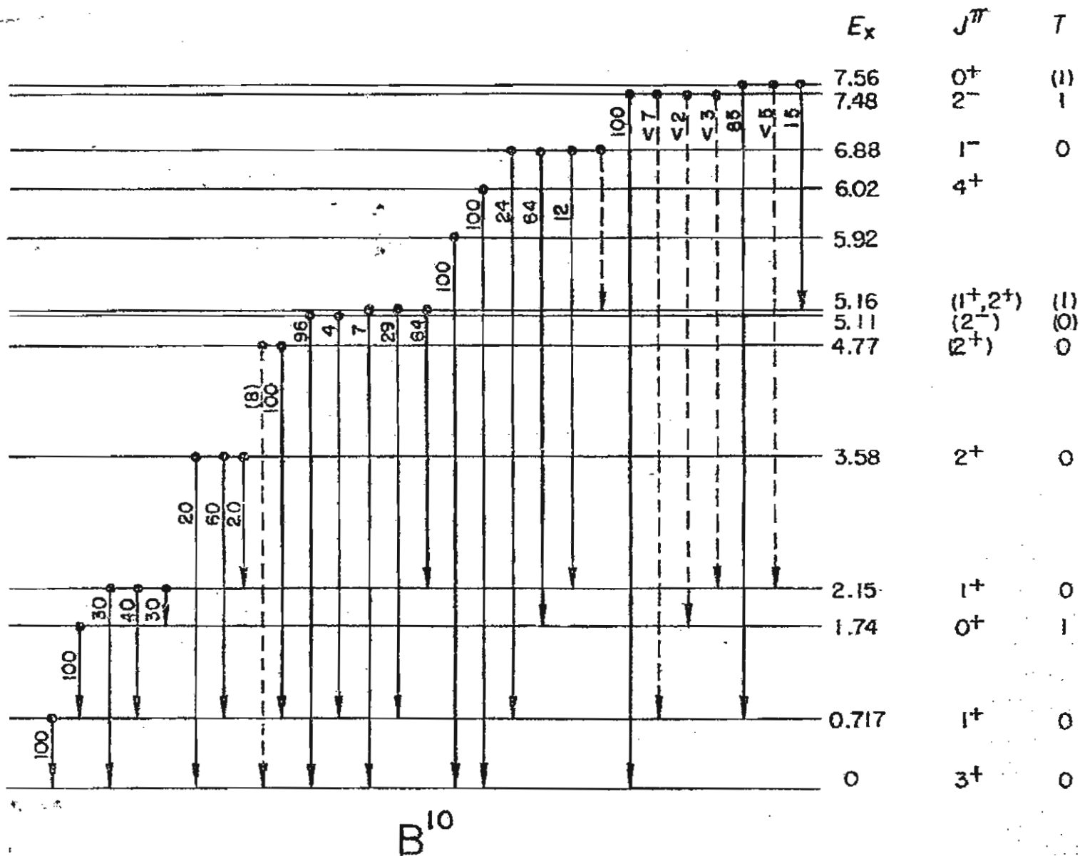
Fig. 14. Gamma-ray transitions in B^{10} . The horizontal lines indicate the pertinent levels of B^{10} , identified on the right by the level energies, and where known, the total angular momentum J , parity, and isobaric spin T . Solid vertical lines indicate observed transitions, while dashed lines indicate transitions whose assignments are not well established. Numbers on the vertical lines give the (estimated) percentage branching from each level; figures in parentheses are least certain.
